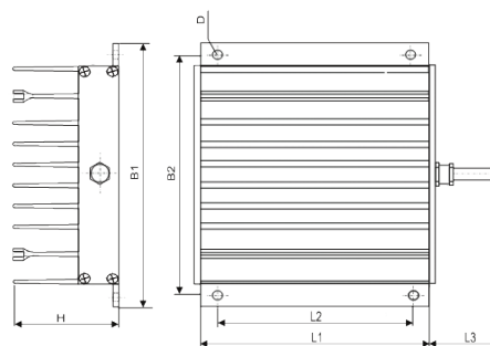
Dimension drawing
