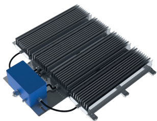
Compact Braking resistor BW 155-combination
