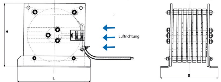
Air choke with disc winding (without cooling unit)
