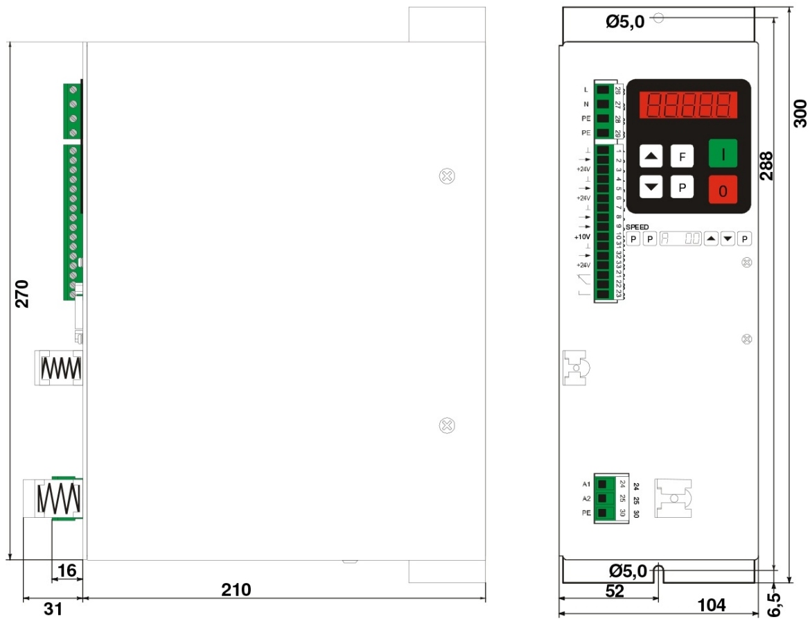
Dimension drawing IP 20 - 16A
